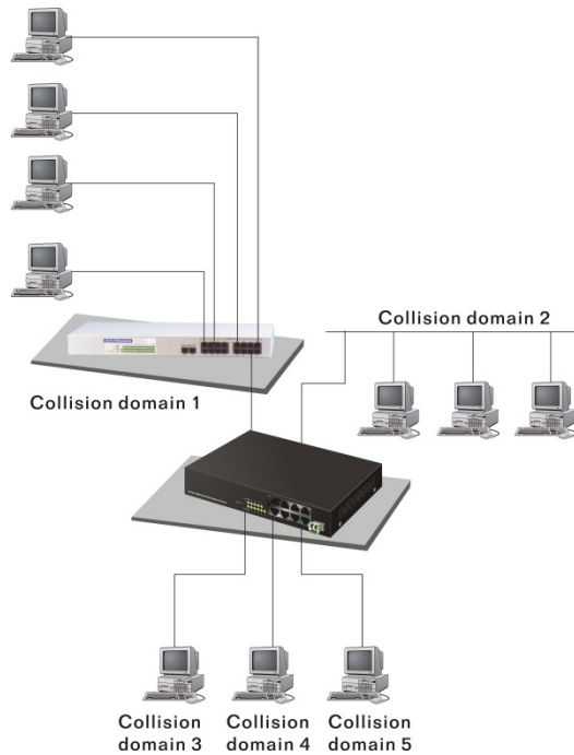
Fig.3-6 Collision Domain
