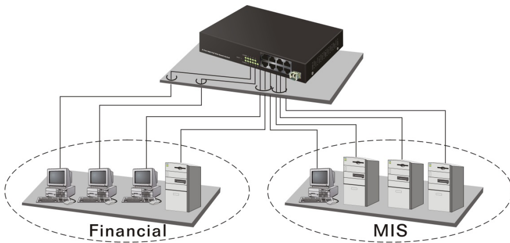
Fig. 2-11 Peer-to-peer Network Connection
