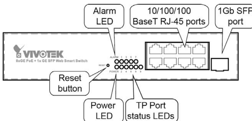
Fig. 1-2 Front View of 9-PORT GBE WEB SMART PoE Switch
