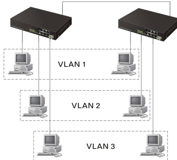
Fig. 2-5 Attribute-based VLAN Diagram
