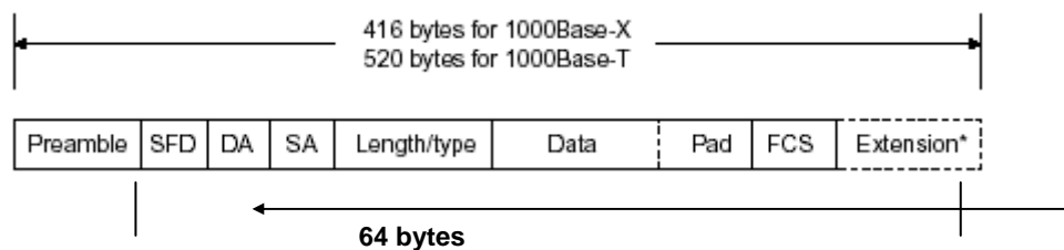
Fig. 3-4 Gigabit Ethernet Frame
