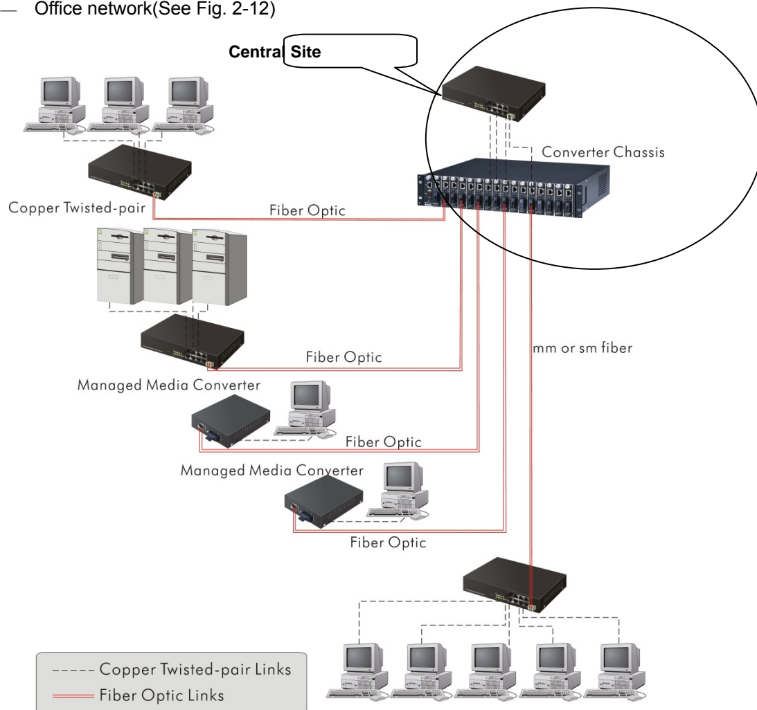
Fig. 2-10 Network Connection between Remote Site and Central Site
