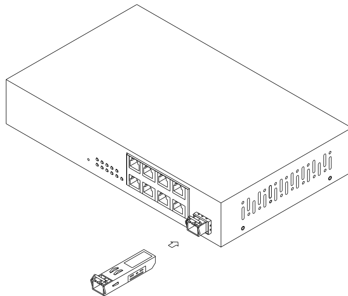
Fig. 2-1 Installation of Optional SFP Fiber Transceiver
